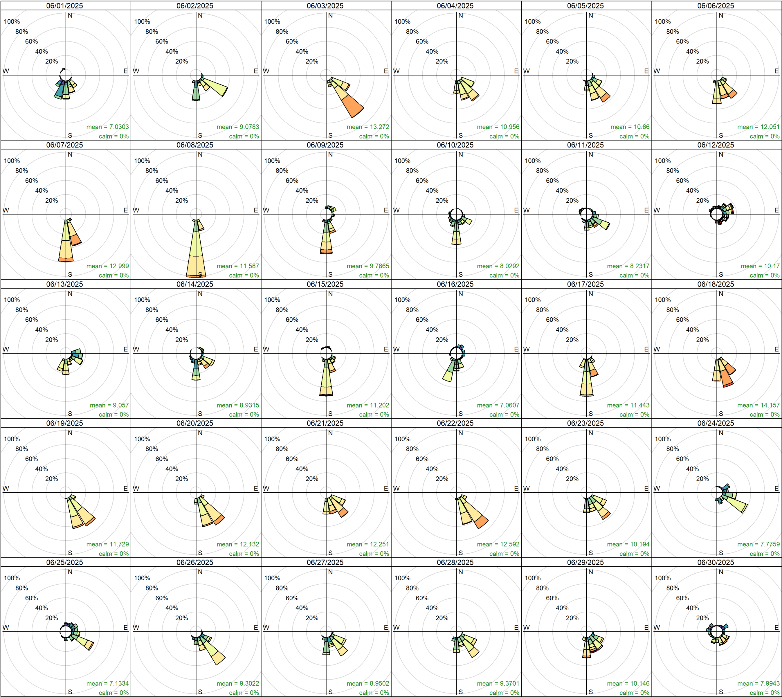
Frequency of counts by wind direction (%)
